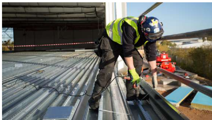
Figure 4.16 Setting out of edge trim
