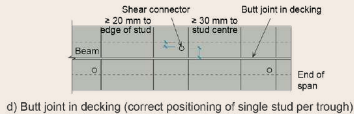
d) Butt joint in decking (correct positioning of single stud per trough)
