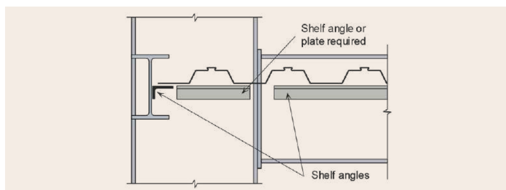
Figure 4.7 Decking support details at a column web
